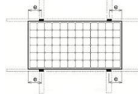
Figure2. Clamping on longer Frame
