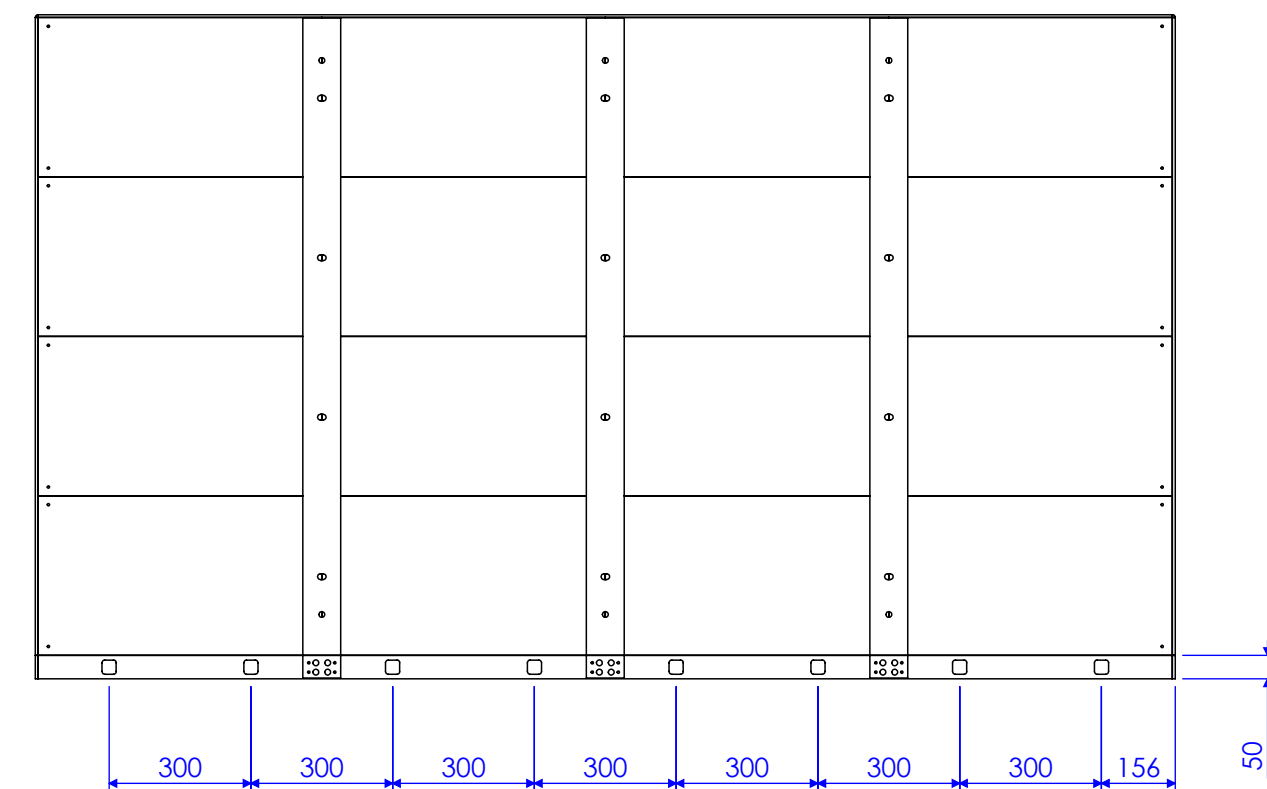
REAR VIEW CABLE HOLES
